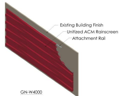
GN-W4000
